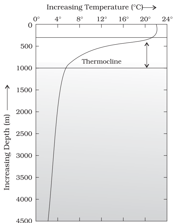
Figure 13.3 : Thermocline
