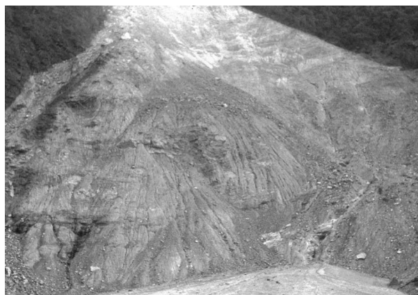
Figure 7.9 : Landslide
